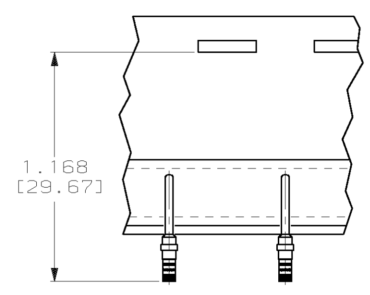
TAPE MOUNTED PART NO 1218371-2 ONLY SCALE 2:1
